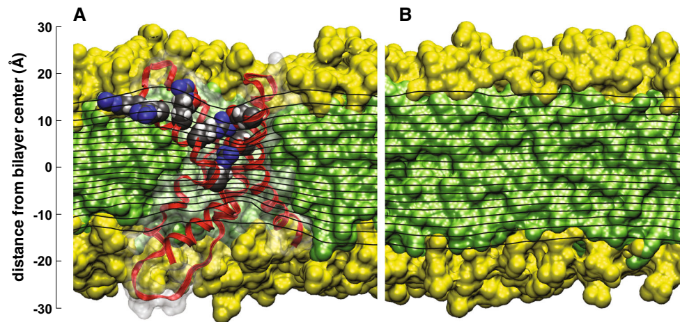
Fig. 5 VSD electrostatics. a The membrane equipotential surfaces (black lines; contour interval is 5 % of the applied potential) on a slice passing through the system center of the VSD show focusing features in the crevices that suggest that charges could be displaced across the membrane electric field over a region that is 65.75 % of the membrane thickness. Contributions to the molecular surface from aliphatic chains (green), polar groups (yellow), and proteins (white, transparent) of the corresponding cut-away view are shown as background. The voltage-sensing domain is in ribbon representation
