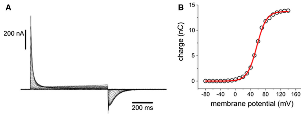
Fig. 1 Electrical characterization of voltage-sensing motions. a Gating (or sensing) currents from the Ciona intestinalis voltage-sensing phosphatase C363S mutant expressed in Xenopus oocytes. The membrane potential was initially held at -60 mV, and ON sensing currents (upward deflections) were elicited by depolarizing to a potential in the range of -80 to +140 mV using 800-ms test pulses. OFF sensing currents were recorded after repolarization to -60 mV.
