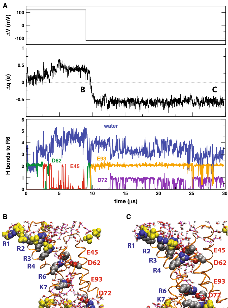
Fig. 6 Gating charge displacement from an all-atom simulation of the VSD of KvAP in a lipid bilayer under an applied electric field. a (upper panel) Time dependence of applied membrane potential, \Delta V , relative to the intracellular side of the membrane. (middle panel) Total charge displacement within the membrane electric field with respect to the initial configuration. Switching the membrane potential from a depolarizing to a repolarizing potential after 9 \mu\text{s} produces 1e of net gating charge. (lower panel) Changes in the solvation environment of R6 as the side chain moves from the center of the VSD into the extracellular cavity (under a depolarizing potential) and from the extracellular cavity to the intracellular cavity (under a repolarizing potential). (b, c) Snapshots of the VSD at two membrane potentials: b Depolarized ( \Delta V = +120\text{mV} ) VSD after 8.5 \mu\text{s} . R4-K7 are shifted outwards with respect to the unpolarized trajectory. c Repolarized ( \Delta V = -120\text{mV} ) VSD after 28.35 \mu\text{s} . The labels in
