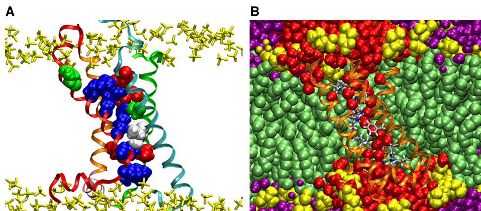
Fig. 4 VSD structure and solvation. Snapshots from a 12 \mu s all-atom simulation of the VSD of the Kv1.2 paddle-chimera channel (Long et al. 2007) in a lipid bilayer in excess water. a The VSD architecture houses two clusters of basic and acidic side chains separated by two hydrophobic residues. The residues determined by Palovcak et al. (2014) to be evolutionary “constrained” are shown as filled-spheres (basic, blue ; acidic, red ; polar, green ; hydrophobic, white . See Fig. 3 for detailed sequence). The VSD is shown in ribbon representation
