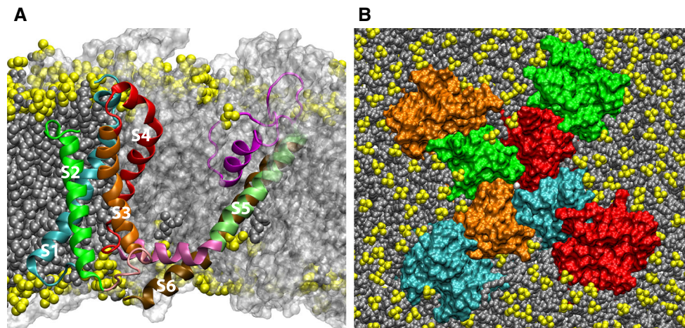
Fig. 2 The structure of the K_v1.2 paddle-chimera channel (Long et al. 2007) in a lipid bilayer. a Cut-away view highlighting a single protein chain colored by transmembrane segment (S1, cyan; S2, green; S3, orange; S4, red; S5 lime; S6, ochre). The connecting region between S1 and S2 is not shown for clarity. The other three protein chains are shown in a transparent molecular surface representation colored white. Lipids are shown as filled-spheres with the headgroups in yellow. b Top view. The pore domain results from the
